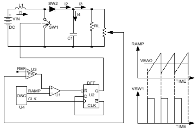
Figure 4. Typical Trailing Edge Control Scheme
